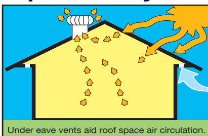
Under eave vents aid roof space air circulation.
